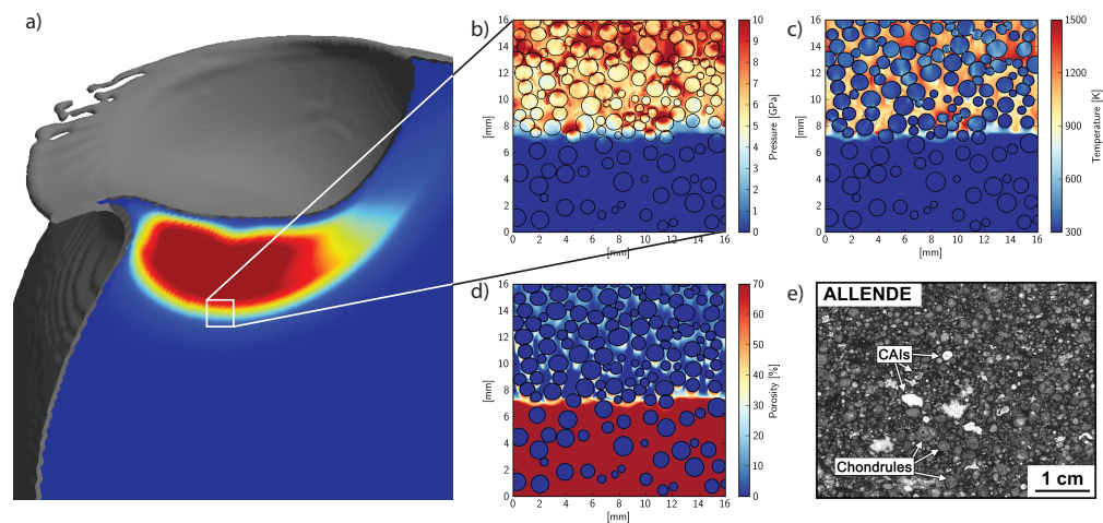
Figure 1: (a) A numerical simulation of an oblique collision between planetesimals. This slice through the centre of the planetesimal shows the bulk shock pressure at one instant during impact. To relate these large-scale conditions to meteorite samples (e.g., (e)) mesoscale simulations of shock compaction examine spatial heterogeneity in: (b) shock pressure; (c) temperature; (d) and porosity. Observe the strong temperature dichotomy between chondrules and matrix owing to the high compaction of matrix porosity, which is incomplete only in the lee of chondrules. (e) An example meteorite sample, showing the heterogeneous nature of a typical meteorite, with abundant chondrules and matrix.
